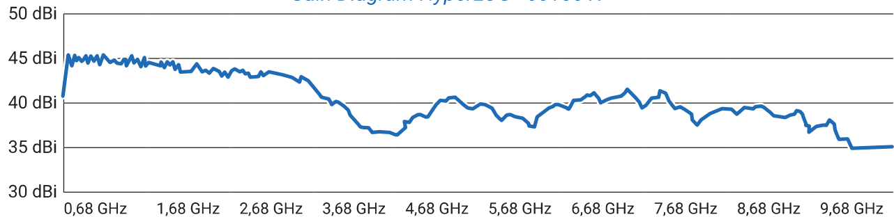
Gain Diagram HyperLOG® 60100 X
