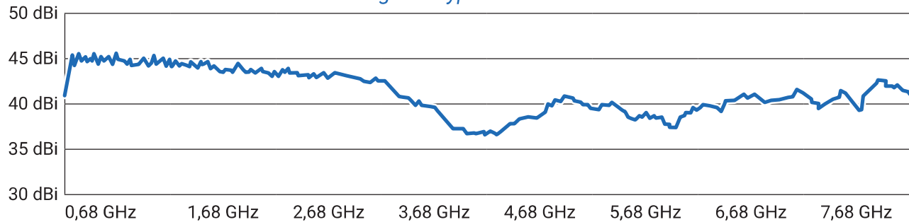
Gain Diagram HyperLOG® 6080 X
