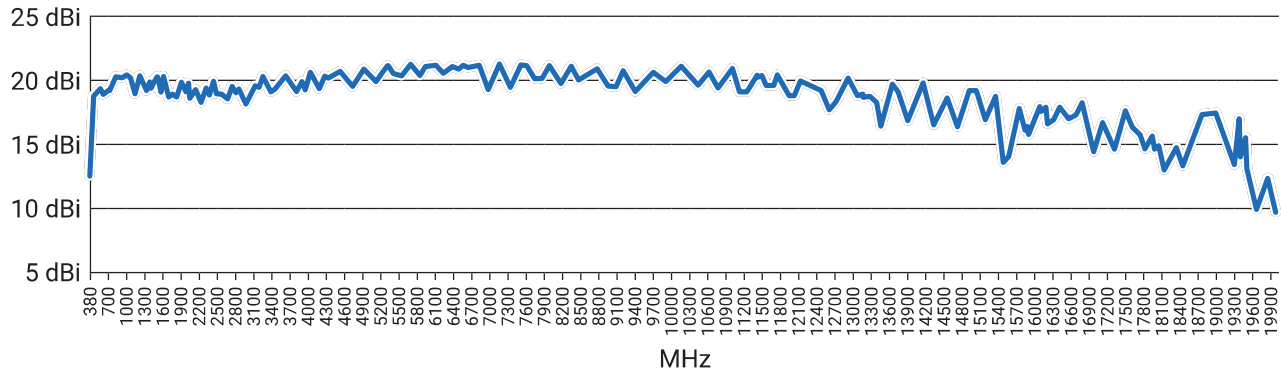
Gain Diagram HyperLOG® 30200 X
