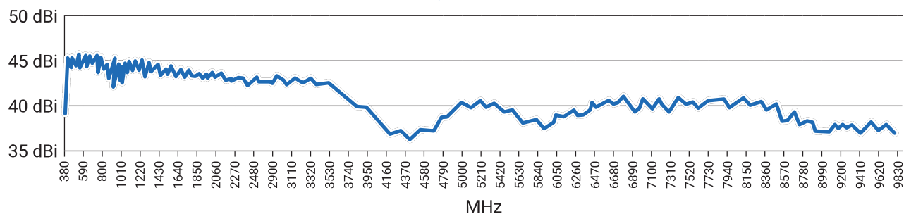
Gain Diagram HyperLOG® 30100 X
