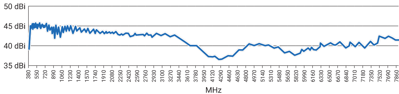
Gain Diagram HyperLOG® 3080 X
