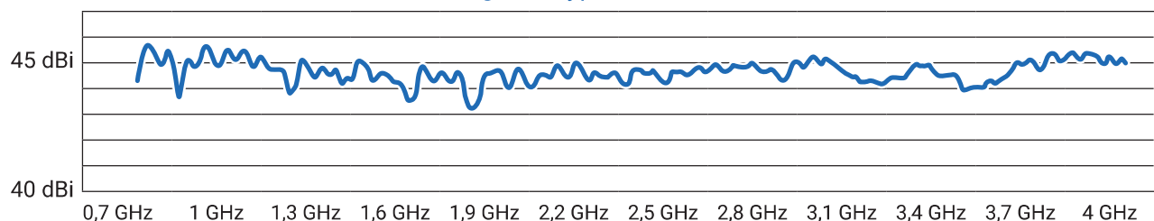
Gain Diagram HyperLOG® 7040 X
