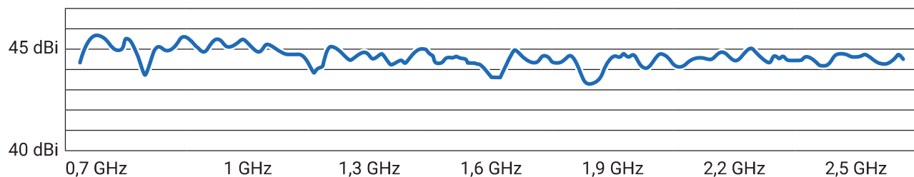
Gain Diagram HyperLOG® 7025 X
