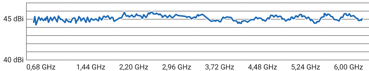
Gain Diagram HyperLOG® 7060 X
